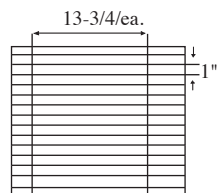
15 Cell Arrangement Max Cell size 13-3/4 x 1 x 6-1/4" 2 Short Partitions - 4 Long Partitions
