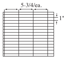
45 Cell Arrangement Max Cell size 5-3/4 x 1 x 6-1/4" 4 Short Partitions - 14 Long Partitions
