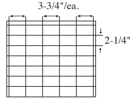
35 Cell Arrangement Max Cell size 3-3/4 x 2-1/4 x 6-1/4" 6 Short Partitions - 7 Long Partitions
