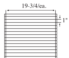
15 Cell Arrangement Max Cell size 19-3/4 x 1 x 6-1/4" 2 Short Partitions - 14 Long Partitions
