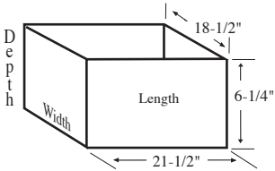
45 Cell Arrangement Max Cell size 5-3/4 x 1 x 6-1/4" 4 Short Partitions - 14 Long Partitions
