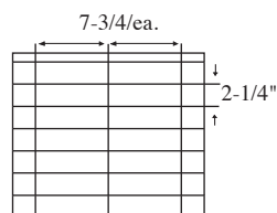
14 Cell Arrangement Max Cell size 7-3/4 x 2-1/4 x 6-1/4" 3 Short Partitions - 7 Long Partitions
