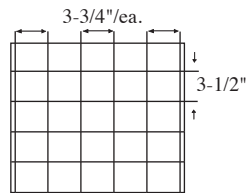
25 Cell Arrangement Max Cell size 3-3/4 x 3-1/2 x 6-1/4" 6 Short Partitions - 4 Long Partitions
