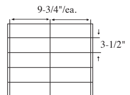
10 Cell Arrangement Max Cell size 9-3/4 x 2-1/4 x 6-1/4" 3 Short Partitions - 4 Long Partitions
