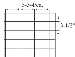
15 Cell Arrangement Max Cell size 5-3/4 x 3-1/2 x 6-1/4" 4 Short Partitions - 4 Long Partitions
