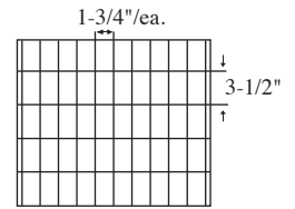
50 Cell Arrangement Max Cell size 1-3/4 x 3-1/2 x 6-1/4" 11 Short Partitions - 4 Long Partitions
