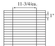
15 Cell Arrangement Max Cell size 11-3/4 x 1 x 6-1/4" 2 Short Partitions - 14 Long Partitions
