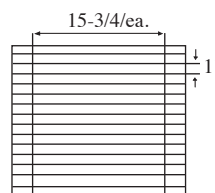
15 Cell Arrangement Max Cell size 15-3/4 x 1 x 6-1/4" 2 Short Partitions - 14 Long Partitions
