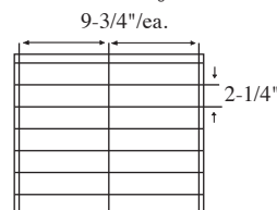
14 Cell Arrangement Max Cell size 9-3/4 x 2-1/4 x 6-1/4" 3 Short Partitions - 7 Long Partitions
