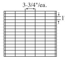
75 Cell Arrangement Max Cell size 3-3/4 x 1 x 6-1/4" 6 Short Partitions - 14 Long Partitions
