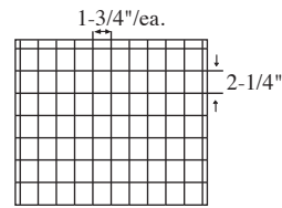
70 Cell Arrangement Max Cell size 1-3/4 x 2-1/4 x 6-1/4" 11 Short Partitions - 7 Long Partitions
