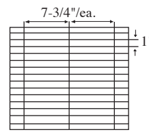
30 Cell Arrangement Max Cell size 7-3/4 x 1 x 6-1/4" 3 Short Partitions - 14 Long Partitions
