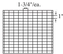
150 Cell Arrangement Max Cell size 1-3/4 x 1 x 6-1/4" 11 Short Partitions - 14 Long Partitions
