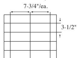
10 Cell Arrangement Max Cell size 7-3/4 x 3-1/2 x 6-1/4" 3 Short Partitions - 4 Long Partitions
