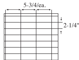
21 Cell Arrangement Max Cell size 5-3/4 x 2-1/4 x 6-1/4" 4 Short Partitions - 7 Long Partitions
