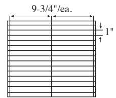
30 Cell Arrangement Max Cell size 9-3/4 x 1 x 6-1/4" 3 Short Partitions - 14 Long Partitions
