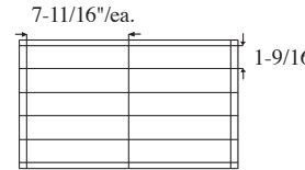
10 Cell Arrangement Max Cell size 7-11/16 x 1-9/16 x 2-3/4" 3 Short Partitions - 6 Long Partitions
