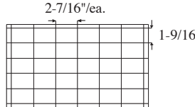
18 Cell Arrangement Max Cell size 2-7/16 x 1-9/16 x 2-3/4" 7 Short Partitions - 6 Long Partitions
