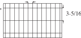
24 Cell Arrangement Max Cell size 3-5/16 x 1-1/8 x 2-3/4" 13 Short Partitions - 3 Long Partitions
