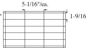
15 Cell Arrangement Max Cell size 5-1/16 x 1-9/16 x 2-3/4" 4 Short Partitions - 6 Long Partitions
