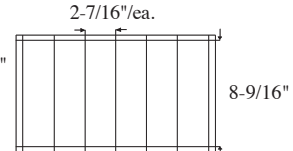
6 Cell Arrangement Max Cell size 8-9/16 x 2-7/16 x 2-3/4" 7 Short Partitions - 2 Long Partitions
