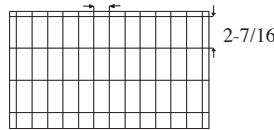
36 Cell Arrangement Max Cell size 2-7/16 x 1-1/8 x 2-3/4" 13 Short Partitions - 4 Long Partitions
