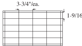
20 Cell Arrangement Max Cell size 3-3/4 x 1-9/16 x 2-3/4" 5 Short Partitions - 6 Long Partitions
