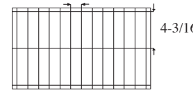
24 Cell Arrangement Max Cell size 4-3/16 x 1-1/8 x 2-3/4" 13 Short Partitions - 3 Long Partitions
