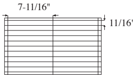
20 Cell Arrangement Max Cell size 7-11/16 x 11/16 x 2-3/4" 3 Short Partitions - 11 Long Partitions
