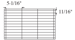
30 Cell Arrangement Max Cell size 5-1/16 x 11/16 x 2-3/4" 4 Short Partitions - 11 Long Partitions
