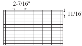
60 Cell Arrangement Max Cell size 2-7/16 x 11/16 x 2-3/4" 7 Short Partitions - 11 Long Partitions
