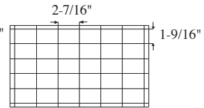
30 Cell Arrangement Max Cell size 2-7/16 x 1-9/16 x 2-3/4" 7 Short Partitions - 6 Long Partitions
