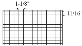
120 Cell Arrangement Max Cell size 1-1/8 x 11/16 x 2-3/4" 13 Short Partitions - 11 Long Partitions
