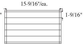
5 Cell Arrangement Max Cell size 15-9/16 x 1-9/16 x 2-3/4" 2 Short Partitions - 6 Long Partitions
