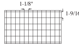
60 Cell Arrangement Max Cell size 1-9/16 x 1-1/8 x 2-3/4" 13 Short Partitions - 6 Long Partitions
