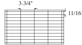
40 Cell Arrangement Max Cell size 3-3/4 x 11/16 x 2-3/4" 5 Short Partitions - 11 Long Partitions
