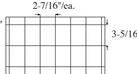
12 Cell Arrangement Max Cell size 3-5/16 x 2-7/16 x 2-3/4" 7 Short Partitions - 11 Long Partitions
