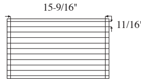
10 Cell Arrangement Max Cell size 15-9/16 x 11/16 x 2-3/4" 2 Short Partitions - 11 Long Partitions
