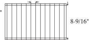
12 Cell Arrangement Max Cell size 8-9/16 x 1-1/8 x 2-3/4" 13 Short Partitions - 2 Long Partitions
